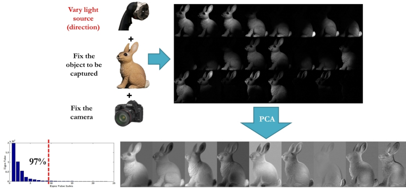
Figure 1.4: The linear subspace which represent all possible images of a specific object under all illumination conditions, while pose kept fixed, can be constructed by performing principal component analysis (PCA) on a large set of images of an object under different illumination conditions. The CVIP Lab bunny was imaged with fixed pose and fixed camera, while the light direction was varied. The light source (coated torch with a tiny hole in the middle to narrow down the light rays in order to simulate a delta function, i.e. single directional light source) was kept at a large distance compared to the object size to simulate distant/directional light source. PCA was then performed using 24 images with different light source directions. The eigenvalue spectrum is shown on the bottom left where nine-basis are found to maintain 97% of image variability, emphasizing low-dimensional representation of images of known object with fixed pose and camera but under arbitrary lighting conditions. This complies with the results of [6] and [7].
