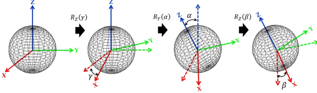
Figure 3.10: Illustration of 3D rotation using Euler angles.
