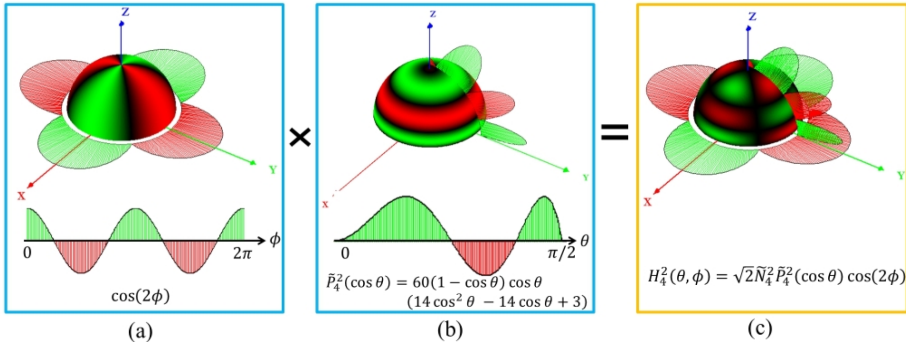
Figure 4.1: An illustration of a real hemispherical harmonic basis function with order/band-index n = 4 and degree m = 2 . (a) The azimuthal part, \cos(2\phi) . (b) The polar part \tilde{P}_4^2(\cos \theta) , which is a shifted associated Legendre polynomial having \theta mapped to the interval [0, 1] through 2 \cos \theta - 1 . (c) The hemispherical harmonic basis resulted from combining the azimuthal and the polar parts with a normalization factor \sqrt{2} \tilde{N}_4^2 . Notice that textured unit hemisphere is used to visualize the hemispherical functions where the greenish and reddish regions correspond to positive and negative values, respectively.
