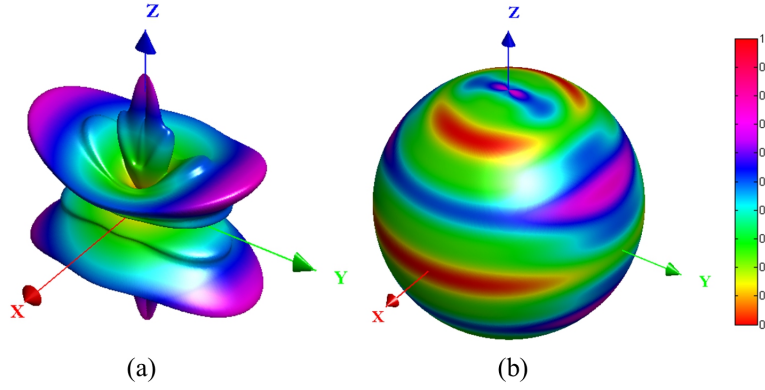
Figure 10.2: An example of spherical function, f^s(\theta, \phi) = \frac{1}{4} [\cos^3(6\theta) + \sin^4(\phi) + 1] visualized as (a) a unit sphere being deformed such that the distance between the sphere's center and the surface points encodes the function absolute values at different spherical coordinates, this is accomplished by the relation between the spherical and cartesian coordinates, (b) a textured unit sphere where the color of its surface points encodes the function values. Note that \theta \in [0, \pi] and \phi \in [0, 2\pi] .
