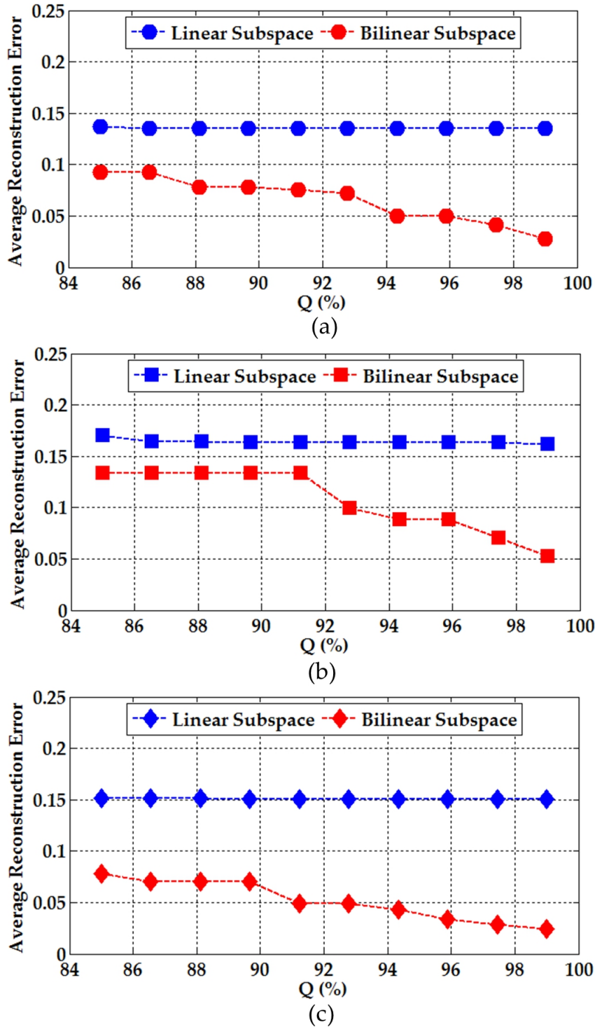
Figure 6.4: The average reconstruction error as a function of the harmonic variation percentage ( Q\% ) maintained by the subspace. Averages were computed based on the 100 rendered testing images for 50 randomly drawn materials from the Merl BRDF database. Surface reflectance is represented using (a) spherical harmonics basis [7], (b) hemispherical Zernike-based basis [44] and (c) the proposed isotropic hemispherical harmonics (HSH)-based Helmholtz reflectance basis.
