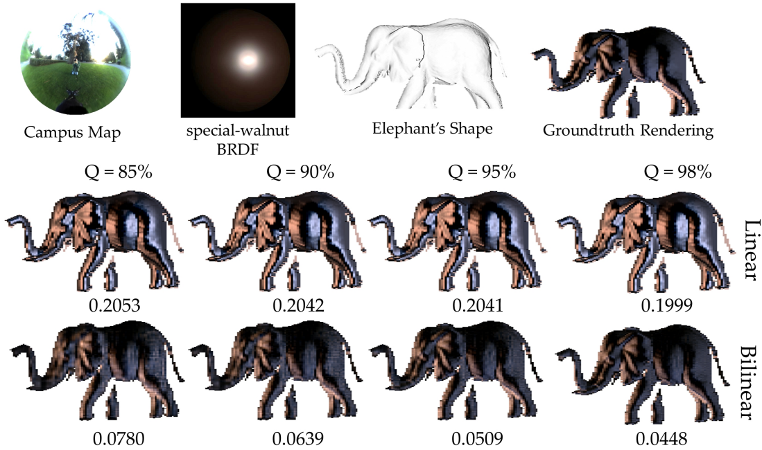
Figure 6.6: Sample reconstructions of the elephant toy from “Weizmann Photometric Stereo Database” [37] using the special-walnut BRDF [17] under the Campus illumination map [55] with different Q(\%) using irradiance harmonics that are based on Zernike-based hemispherical basis deployed by Nilius ad Eklundh in [32, 44]. Mean absolute error (MAE) is shown below each rendered image where all intensities are normalized in the range [0, 1] .
