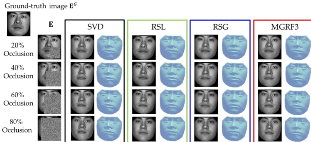
Figure 7.13: Shape and albedo recovery results for one out-of-training sample of Yale Database, where random occluder is used.
