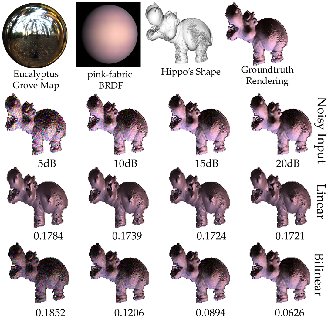
Figure 6.10: Sample reconstructions of the hippo toy from “Weizmann Photometric Stereo Database” [37] using the pink-fabric BRDF [17] under the Eucalyptus Grove illumination map [55] with different SNR levels using irradiance harmonics that are based on Zernike-based hemispherical basis deployed by Nillius ad Eklundh in [32, 44]. Mean absolute error (MAE) is shown below each rendered image where all intensities are normalized in the range [0, 1].
