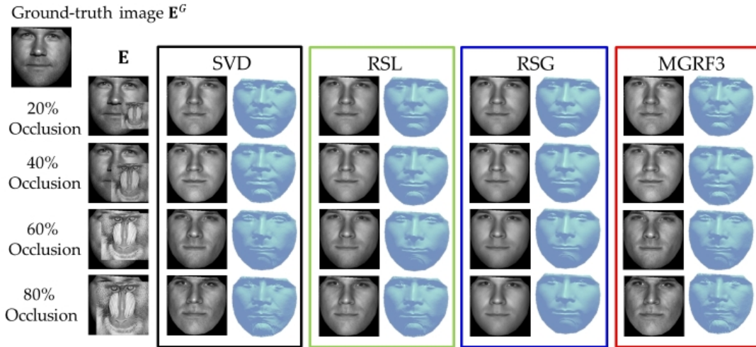
Figure 7.12: Shape and albedo recovery results for one out-of-training sample of Yale Database, where baboon image is used as the occluder.
