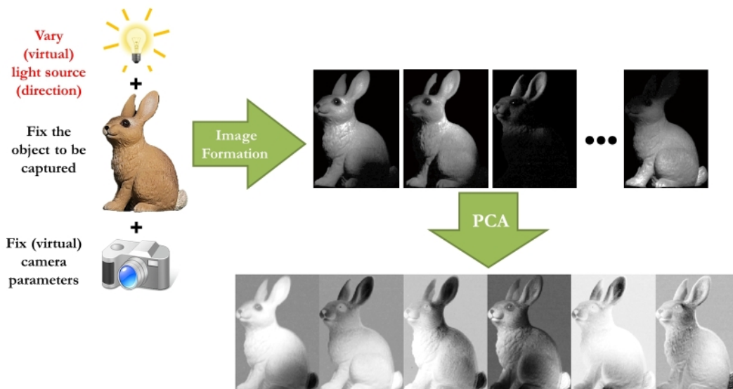
Figure 1.5: The linear subspace which represent all possible images of a specific object under all illumination conditions, while pose is kept fixed, can be constructed by simulating image formation process using 3D models to render synthetic images under various illumination conditions, while PCA is used to compute the required subspace. The Cyberware scanner was used to obtain the shape and albedo of the CVIP Lab bunny.
