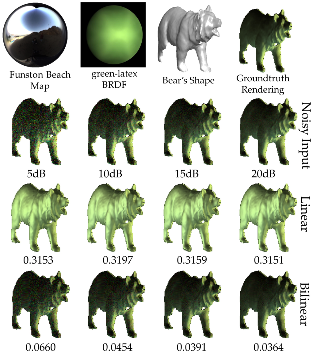
Figure 6.11: Sample reconstructions of the bear toy from “Weizmann Photometric Stereo Database” [37] using the green-latex BRDF [17] under the Funston Beach illumination map [55] with different SNR levels using irradiance harmonics that are based on the proposed Helmholtz HSH-based basis. Mean absolute error (MAE) is shown below each rendered image where all intensities are normalized in the range [0, 1].
