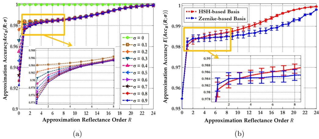
Figure 4.15: The Oren-Nayar BRDF approximation accuracy of the Helmholtz HSH-based basis as a function of the approximating order, where in (a) each curve corresponds to the average approximation accuracy over all sampled incident directions for several values of surface roughness, and in (b) it is compared to Zernike-based basis proposed by Koenderink et al. [21], where the mean and standard deviation were taken over e_N(\sigma) .
