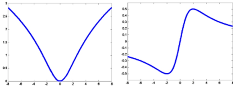
Figure 7.5: Lorentzian \rho and \psi functions. Left: \rho(x) = \log\left(1 + \frac{1}{2}\left(\frac{x}{\sigma}\right)^2\right) . Right: \psi(x) = \rho'(x) = \frac{2x}{2\sigma^2+x^2}
