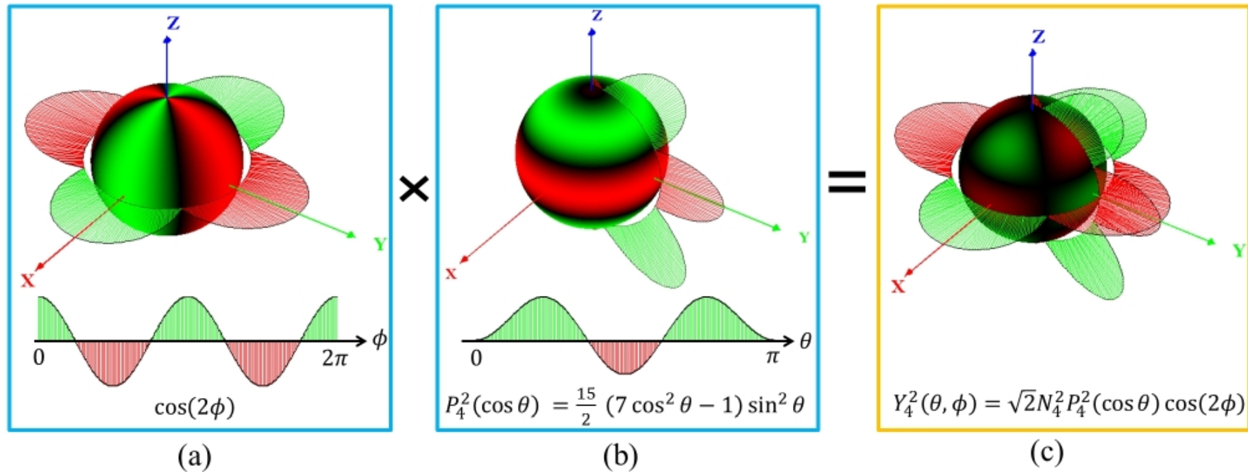
Figure 3.8: An illustration of a real spherical harmonic basis function with order/band-index n = 4 and degree m = 2 . (a) The azimuthal part, \cos(2\phi) . (b) The polar part P_4^2(\cos \theta) , which is an associated Legendre polynomial having \theta mapped to the interval [-1, 1] through \cos \theta . (c) The spherical harmonic basis resulted from combining the azimuthal and the polar parts with a normalization factor \sqrt{2} N_4^2 . Notice that textured unit sphere is used to visualize the spherical functions where the greenish and reddish regions correspond to positive and negative values, respectively.
