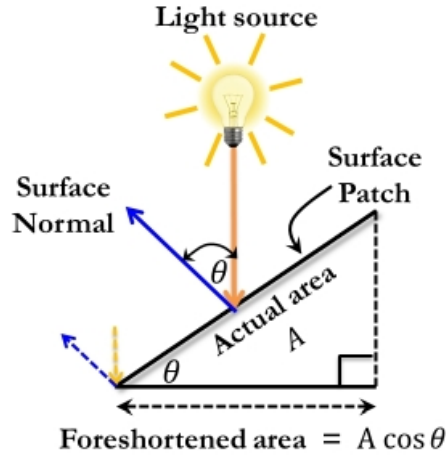
Figure 2.2: A light source sees the foreshortened area of a surface patch instead of its actual area. The foreshortened area depends on the actual area and the angle between the light ray and the surface normal.
