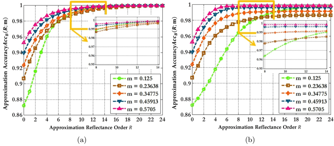
Figure 4.18: The Cook-Torrance BRDF approximation accuracy of (a) the Helmholtz surface reflectance basis, (b) Zernike-based basis, as a function of the approximating order, where each curve corresponds to the average approximation accuracy over all sampled incident directions for several values of surface roughness.
